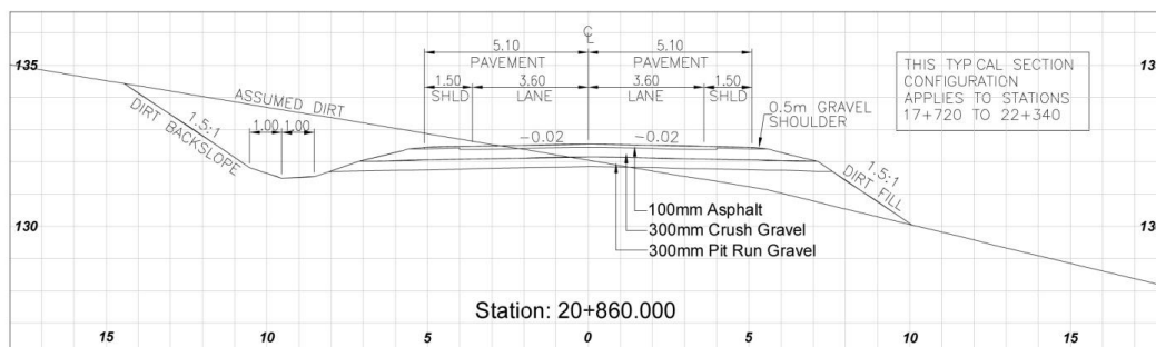
Figure 3.1: Typical Cross Section Ring Road
